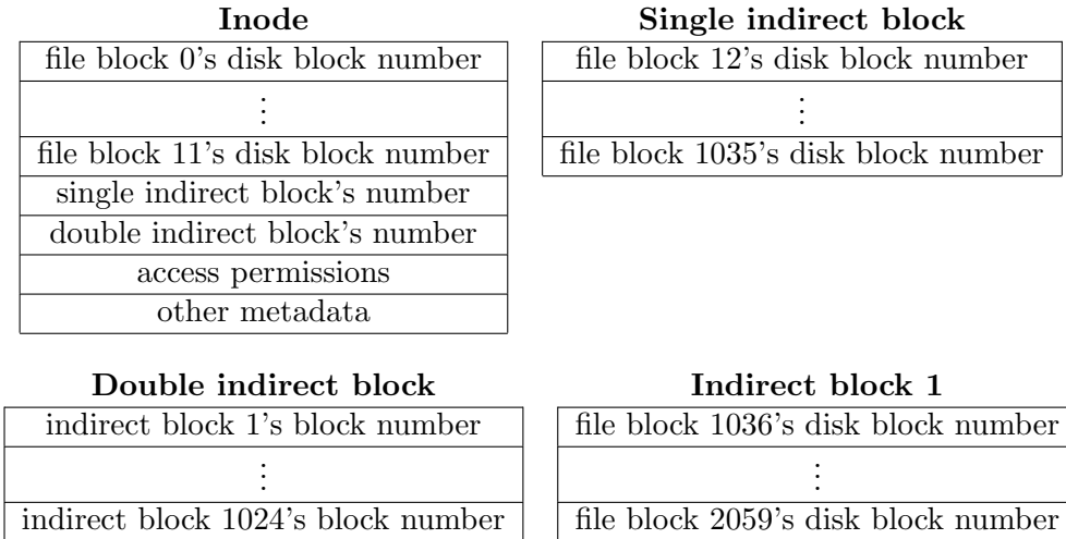
Figure 8.9: If an inode were used with single and double indirect blocks, the block numbers would be stored as shown here.
