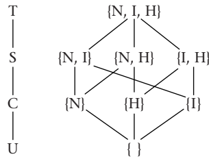
Figure 11.2: The classification levels top secret (T), secret (S), confidential (C), and unclassified (U) form a total order, as shown on the left. Sets of compartments, on the other hand, form only a partial order, namely the subset order in which one set of compartments is below another if it has a subset of the other’s compartments. This is illustrated on the right with three hypothetical compartments: nuclear weapons (N), international terrorism (I), and human intelligence (H). Someone cleared for {I, H}, for example, could read documents labeled with {I, H}, {I}, {H}, or {}.
